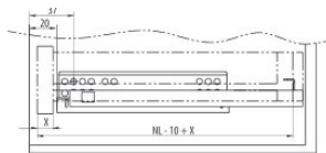
Notranji predal LT min=NL+21
