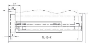
Notranji predal LT min=NL+21
